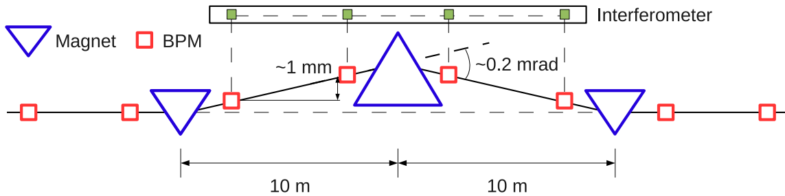
Figure 13. A 3-magnet spectrometer chicane.
