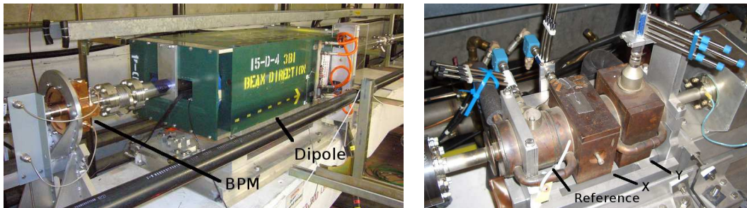
Figure 3. One of the SLAC ILC type BPMs (BPM 5) followed by the first magnet of the chicane (3B1) in the ESA beamline (left), one of the SLAC type BPMs using rectangular cavities (BPM 9) (right).
