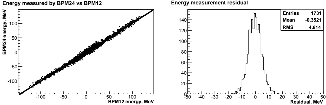
Figure 8. Comparison of BPMs 12 and 24: BPM 24 vs BPM 12 energy measurement (left), residual between BPM 12 and 24 measurements (right).
