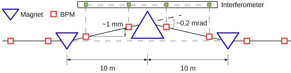
Figure 11. A 3-magnet spectrometer chicane.
