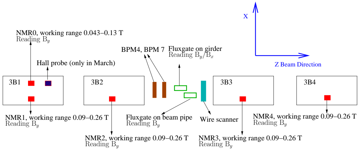
Figure 2. Magnetic field diagnostics in the spectrometer chicane.
