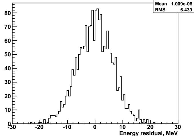
Calibrated residual between BPM24 and 12
