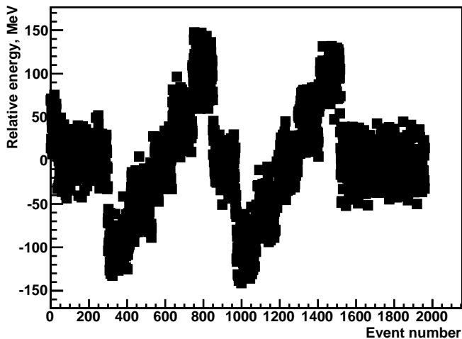
Uncalibrated energy, BPM24 vs BPM12
