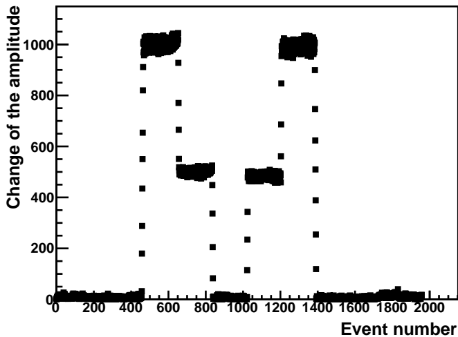
Energy calibration for BPM4
